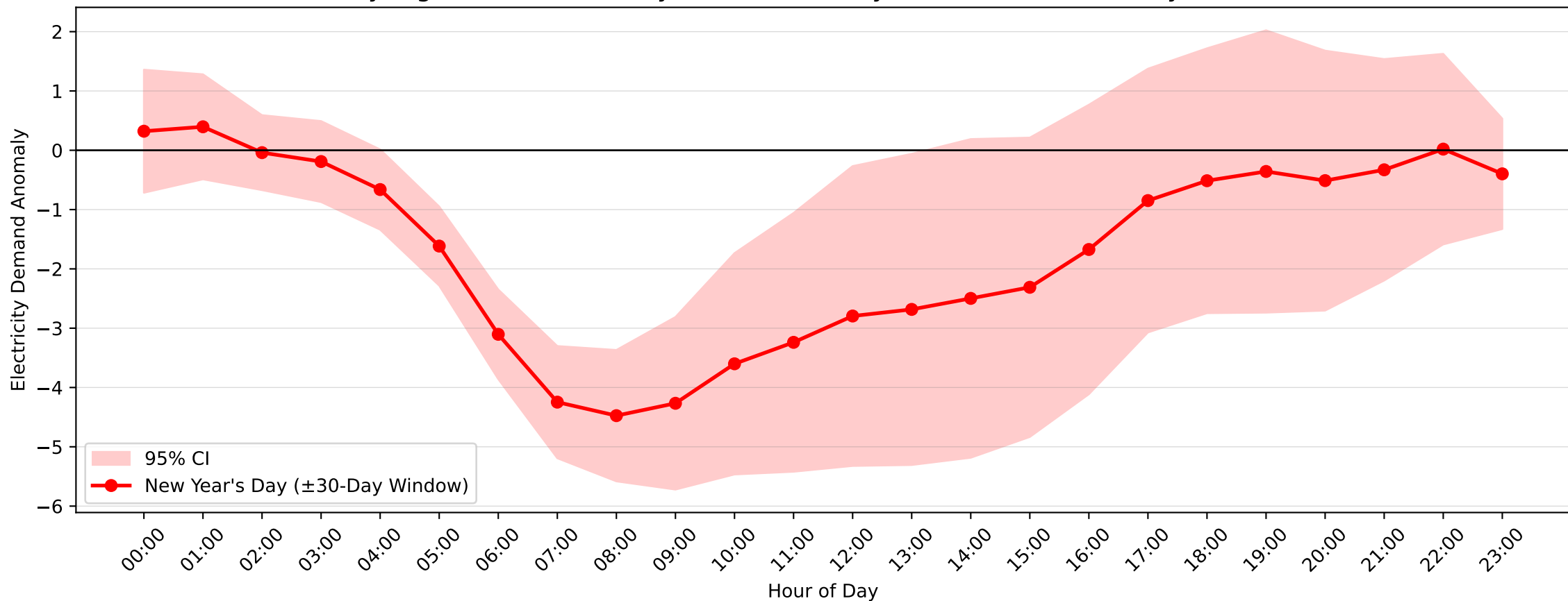
Wyong Demand Anomaly: New Year's Day (2004-2017, \pm 30 -Day Window)
